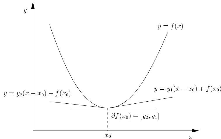
Figure 1: Subdifferential example.
