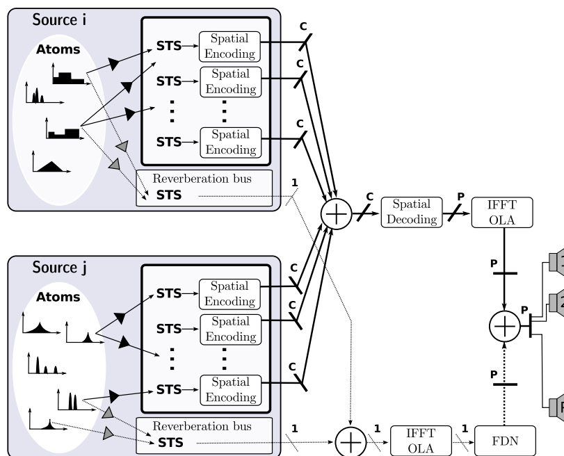
Fig. 2: Architecture of the synthesis/spatialization engine. Deterministic and stochastic components of the atoms are added in the frequency domain to form a collection of spectra (STS) that are spatialized around the listener (spatial encoding/decoding with C intermediate channels). Inverse fast Fourier transform (IFFT) and overlap-add (OLA) are performed to get the multichannel signal for an arbitrary setup of P loudspeakers (or headphones). A supplementary short-time spectrum is dedicated to the reverberation, common for all sources in the scene and implemented by a Feedback Delay Network (FDN) in the time domain (1 input channel, P output channels).
