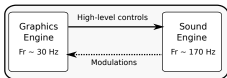
Fig. 5: Audio/graphics interactions. The graphics engine sends high-level designer controls (e.g., fire intensity and position) at the frame rate F_r = 30 Hz. For specific effects, the audio engine may also compute modulation parameters (e.g., flame energy) that are sent back to update the graphics.
