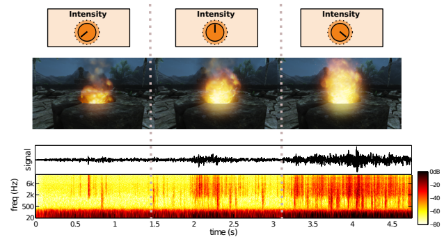
Fig. 3: Audio/graphics high-level control of a fire. The control Intensity changes the rate and gain of noisy impacts, and the combustion noise of the fire sound model. Simultaneously, it controls the flame/smoke particle spawn rate for the graphics simulation.
