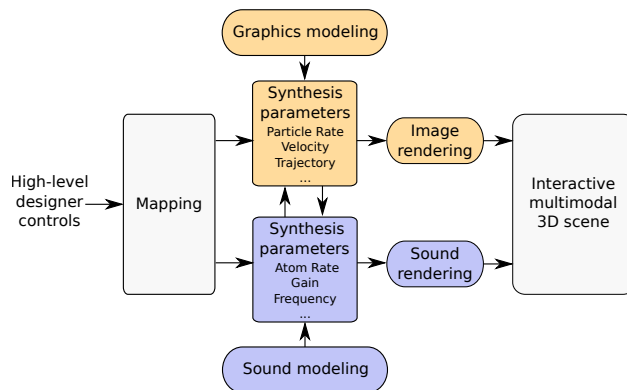
Fig. 1: Environmental sound synthesis for particle-based environmental effects. A mapping between graphics and sound parameters allows tightly-coupled audio/graphics interactions.
