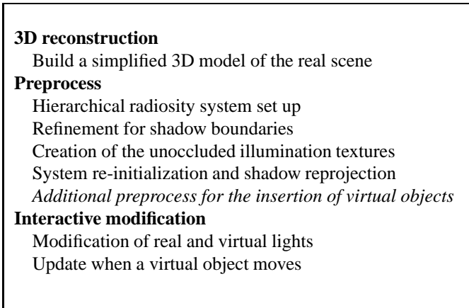
Figure 6: Complete algorithm.
