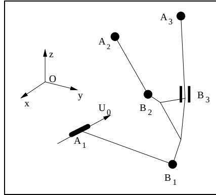
Fig. 3. MacPherson - notations
