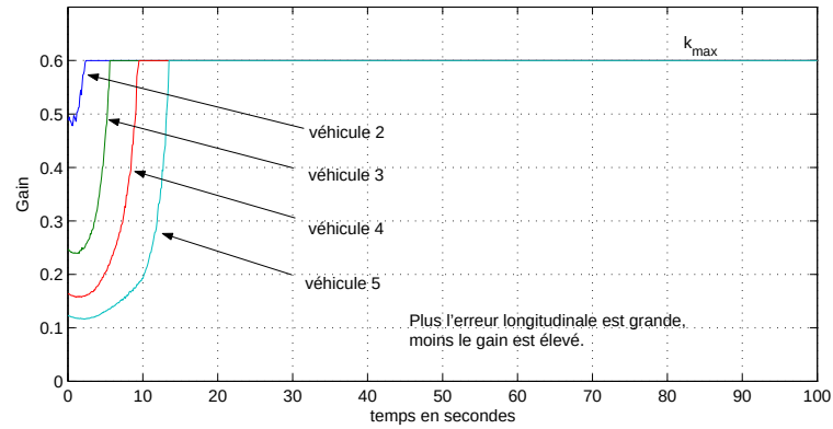
FIG. 2.35 – Gain adaptatif - Simulation 8
