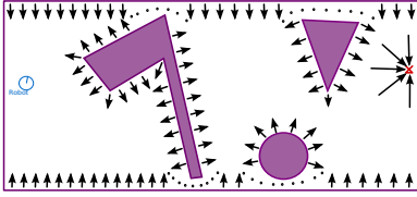
FIGURE 1.17 – Champ de force initial
