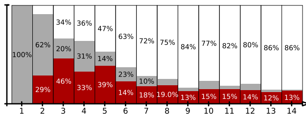
Fig. 10 Percentage of configurations with positive (white), null (gray) and negative (dark red) effects on duration using D-SSA (Color figure online)
