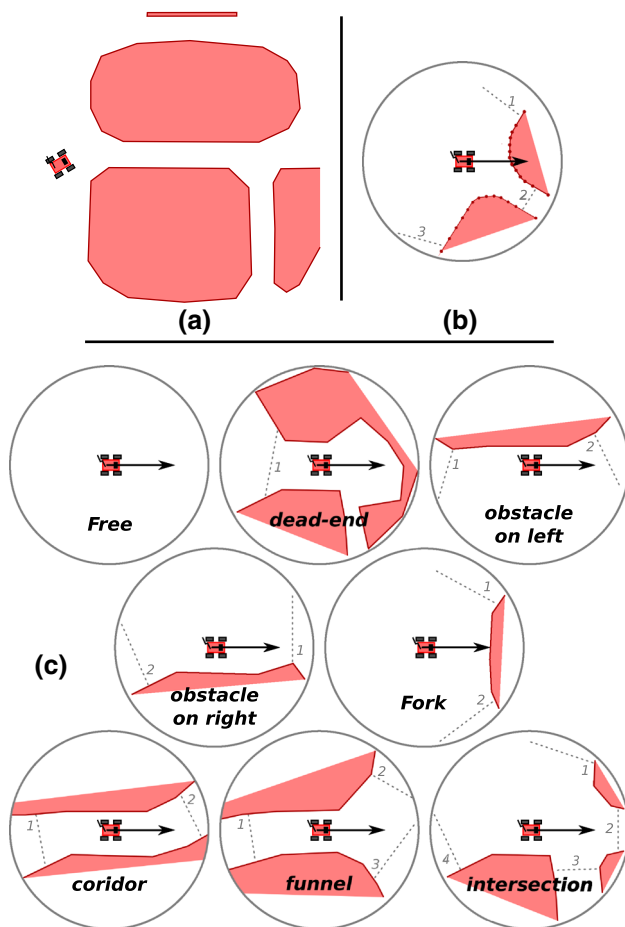
Fig. 2 From local perception to semantic characterization: a the robot in the environment; b the corresponding local model, this configuration has three exits (in gray dotted lines); c the possible eight local semantic states
