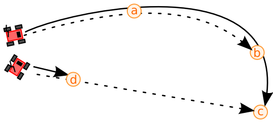
Fig. 4 Minimal movement allocation (dark arrows) versus minimal duration allocation (dotted arrows) with two robots and four goals
