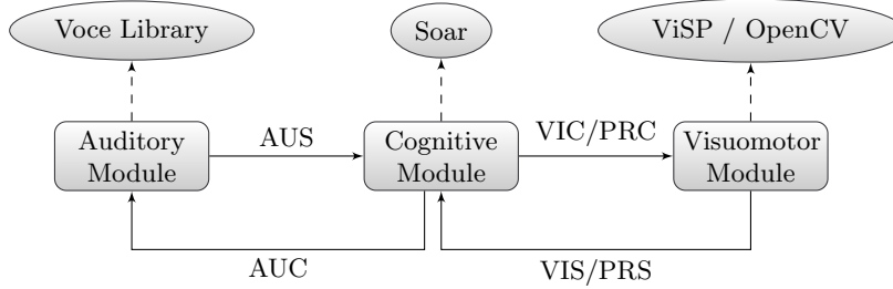
Fig. 2: The CRR architecture. The boxes represent modules and the ovals indicate the libraries wrapped inside the modules. The links between modules indicate topics. AUS: auditory sensory, PRS: proprioceptive sensory, VIS: visual sensory, AUC: Auditory command, VIC: Visual command, PRC: Proprioceptive command.
