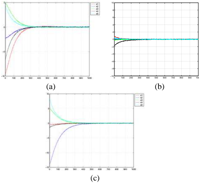
Fig. 6. Hyperbolic mirror-perspective camera ( s - s^* ): (a) Errors for the first conic, (b) Errors for the second conic, (c) Errors for the third conic
