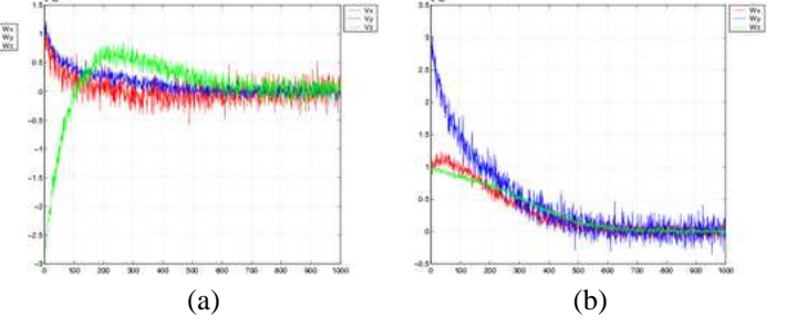
Fig. 8. Parabolic mirror-orthographic camera: (a) Translational velocities [m/s] and (b) rotational velocities [rad/s]
