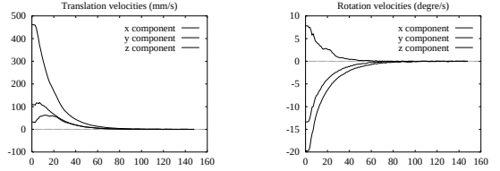
Figure 9: Control vector (\underline{V}, \underline{\Omega})
