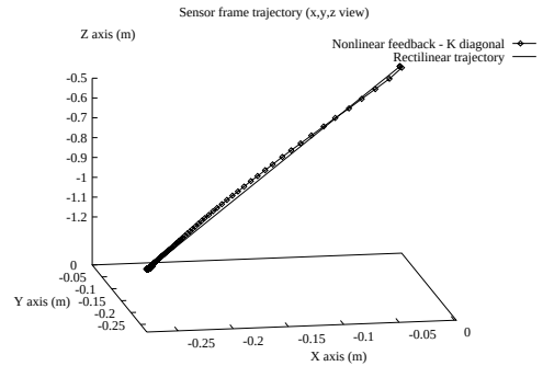
Figure 4: Sensor frame trajectory (scale in m)
