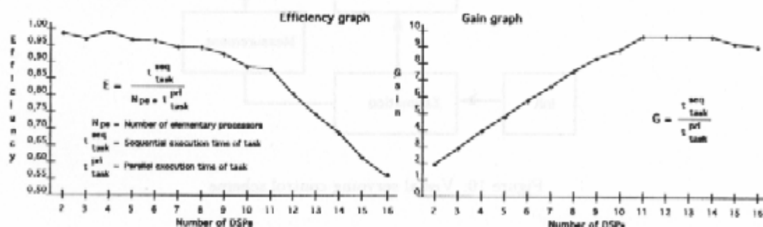
Figure 8: Efficiency and Gain of WINDIS architecture
