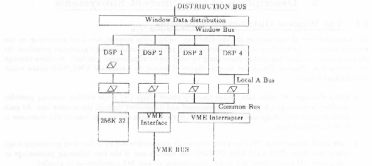
Figure 5: Window processing subsystem overview
