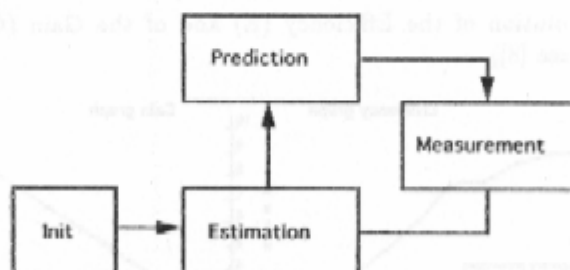
Figure 10: Visual servoing control scheme
