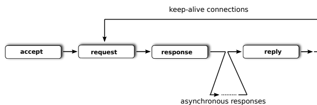
Figure 7. Internal pipeline of the Hop web server with asynchronous responses.
