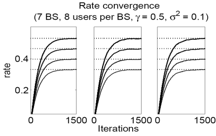
Fig. 2. Rate convergence for Systems S1, S2 and S3 (H1 Network)
