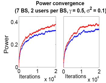
Fig. 6. Power convergence for Systems S4 and S5 (H2 Network)
