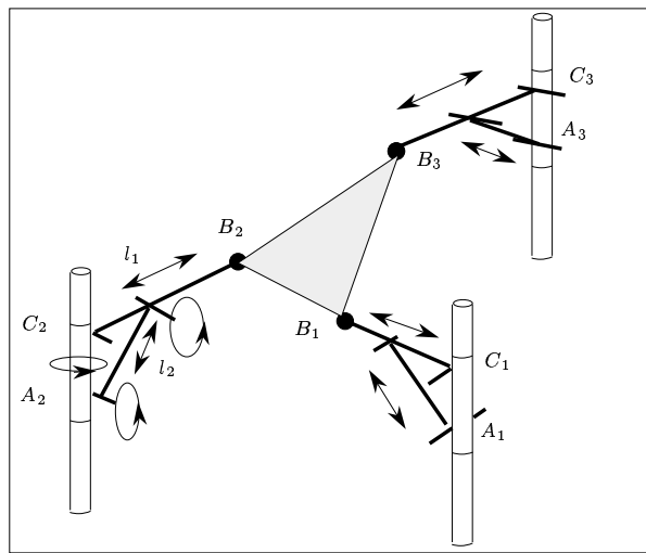
Figure 11: Stewart platform.
