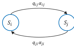
Figure 13: Markov chain.
