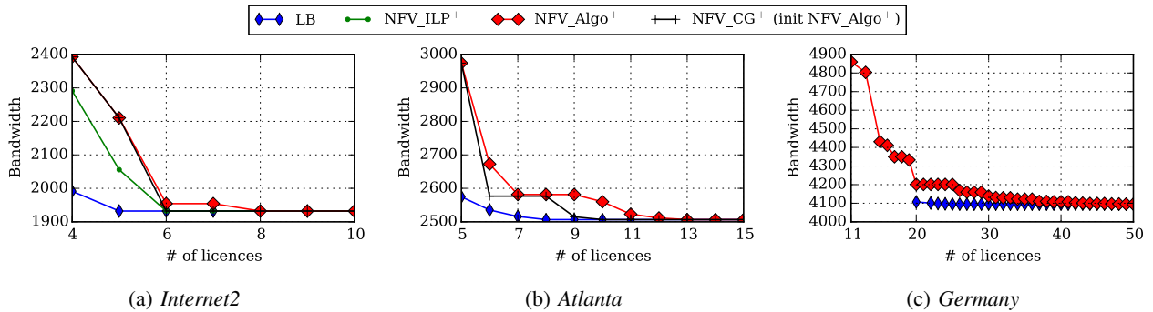
Fig. 9: Bandwidth usage as a function of the number of allowed function replicas.
