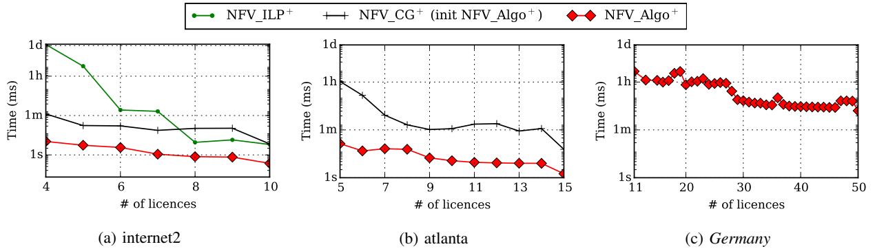
Fig. 6: Execution times of the three methods, the ILP, the column generation model, and the algorithm NFV\_Algo^+ , for different limits on the number of function replicas.
