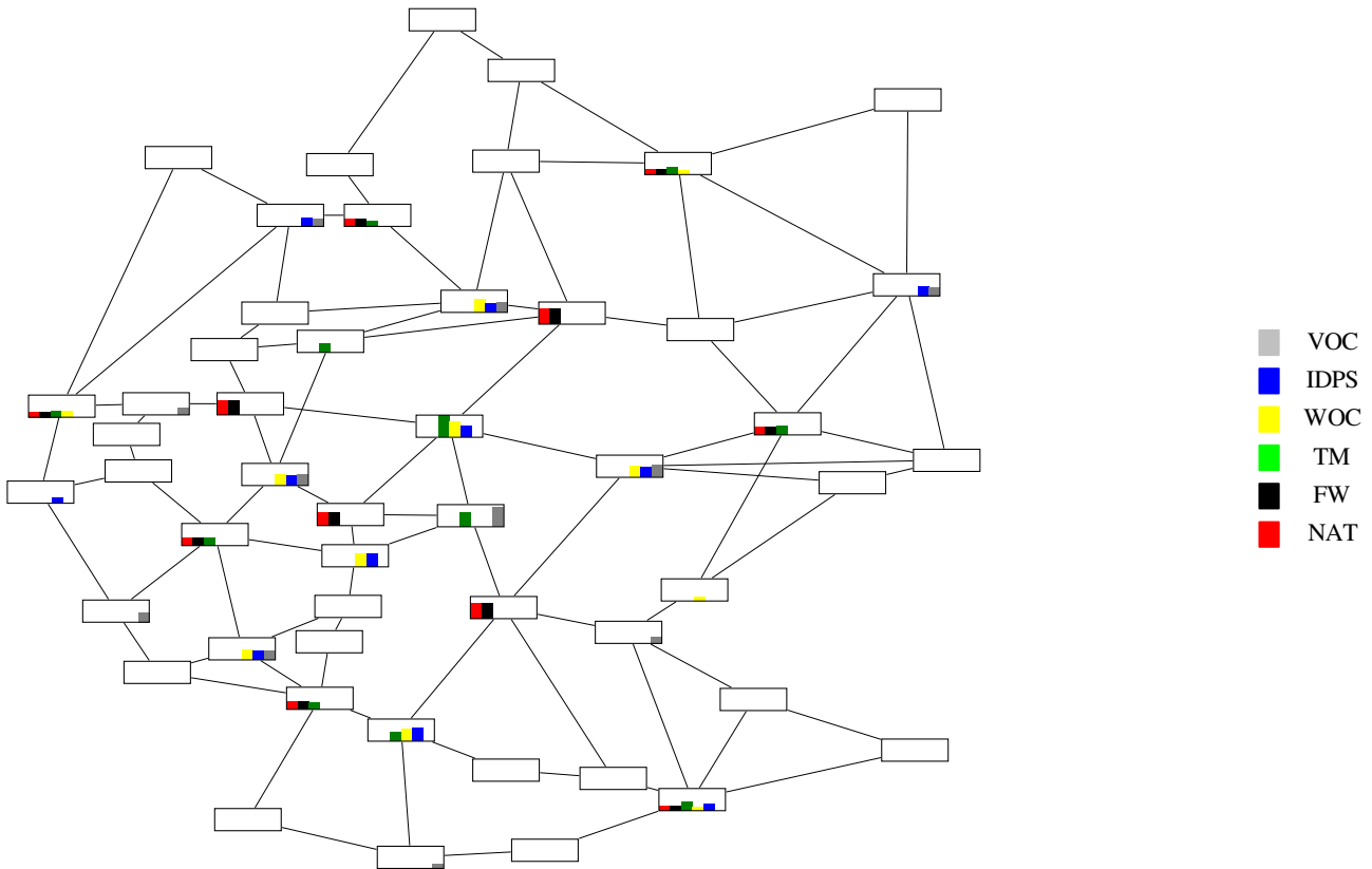
Fig. 8: Placement of functions given by NfV_Algo + when the number of function replicas is limited to 11 for Germany . Bar height in a node gives the percentage of requests (between 0 and 20%) associated with the node function replica
