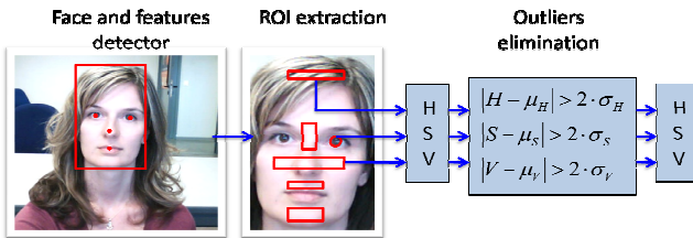
Figure 1. ROI for the bag of facial soft biometrics. Outlier filtering was a function of the standard deviation \sigma and the mean \mu for each of H, S and V.
