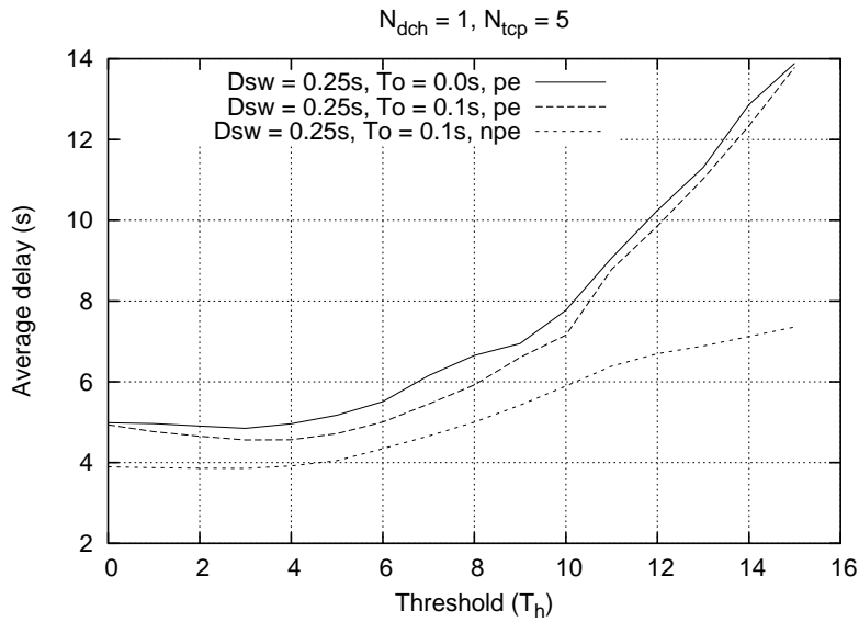
Figure 7.5: Average delay versus T_h . N_{dch} = 1, N_{tcp} = 5, D_w = 250ms .
