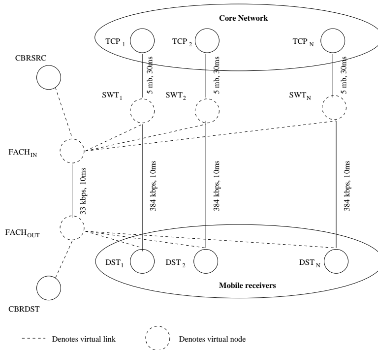
Figure 7.1: Simulation setup
