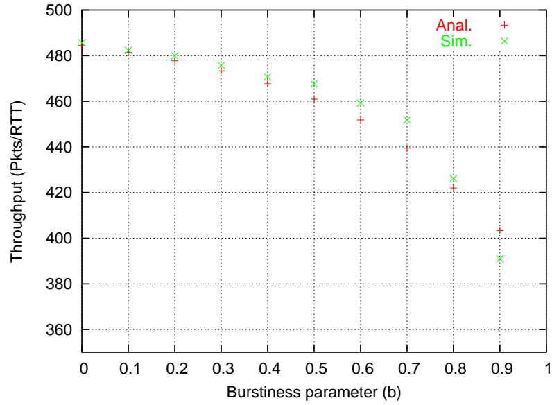
Figure 2.15: Throughput versus burstiness parameter. p_a = 0.02 . W_{max} = 500 .
