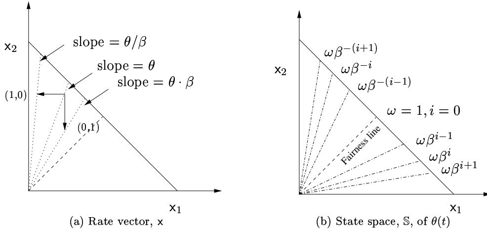
Figure 4.4: Geometric interpretation.
