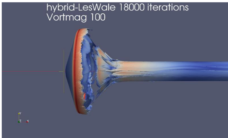
Figure 2: Flow around a probe model at Reynolds number 1 million : Q-criterion isosurfaces.
