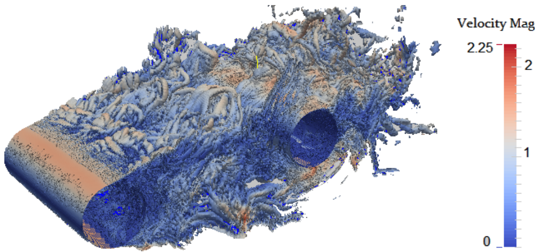
Figure 1: Tandem cylinders at Reynolds number 166000 : instantaneous Q-criterion isosurfaces (colored with velocity modulus).
