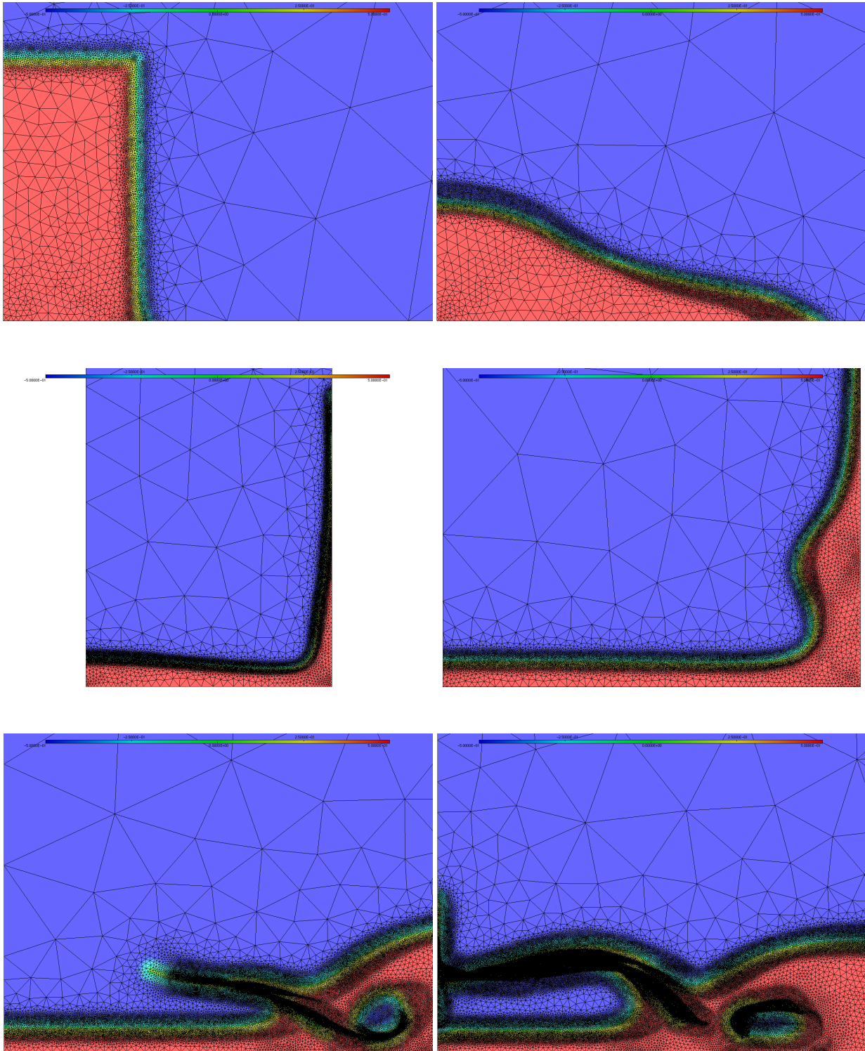
FIG. 5.1 – Chute de la colonne en 2d à t = 0s , t = 0.2s , t = 0.4s , t = 0.6s , t = 0.8s et t = 0.9s .
