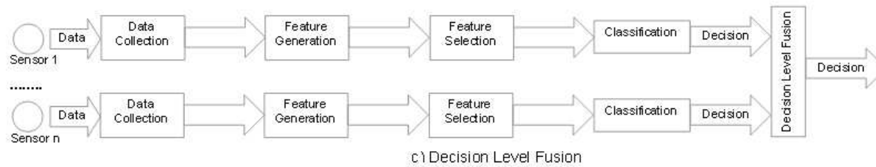
Figure 2.6: Fusion Levels: a) Data Level Fusion; b) Feature Level Fusion; c) Decision Level Fusion; Adapted from Yang et al. [Yang, 2006]
