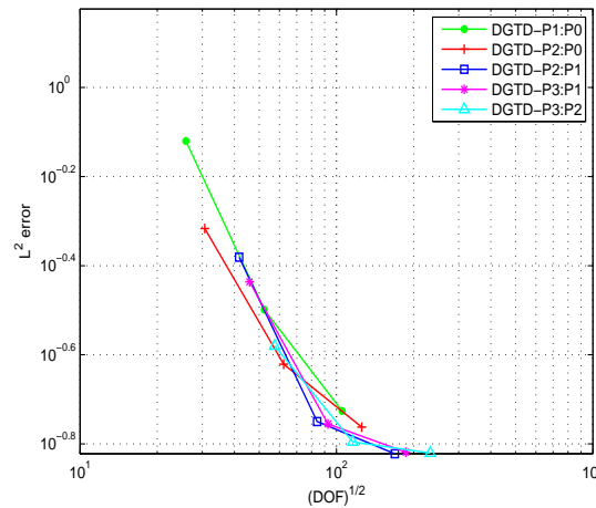
FIG. 3.28 – Scattering of a plane wave by a dielectric cylinder - Configuration S1. Numerical convergence of the hp -refinement DGTD- \mathbb{P}_{p_c}:\mathbb{P}_{p_f} method. Non-conforming triangular meshes.
