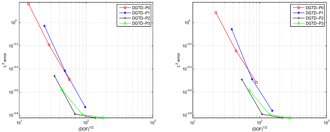
FIG. 3.27 – Scattering of a plane wave by a dielectric cylinder - Configuration S1. Numerical convergence of the h -refinement DGTD- \mathbb{P}_p method. Conforming (left) and non-conforming (right) triangular meshes.
