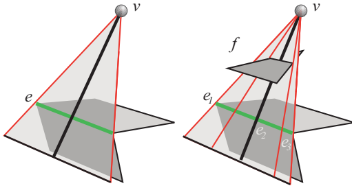
Figure 9: Swath validation. (a) The swath e\nu is valid since the midline does not touch any other object. (b) The swath e_2\nu is invalid, since the midline is blocked by the face f , and the receiver has not been encountered.
