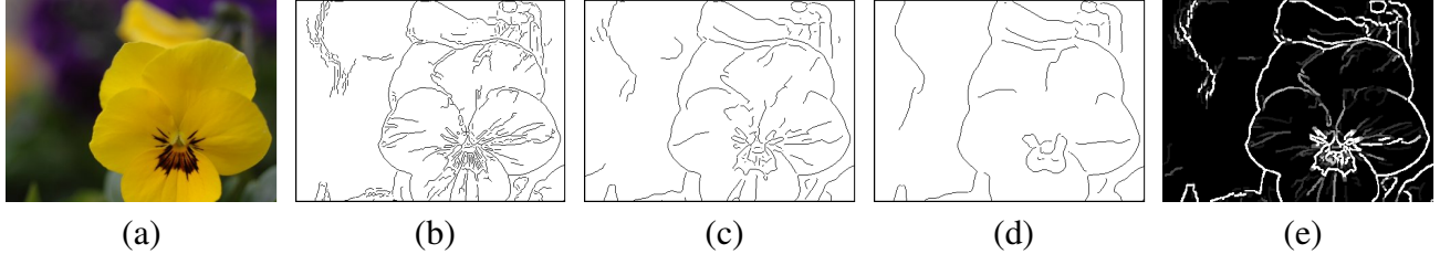
Figure 2.5: Edge importance. (a) The input image. (b-d) Canny edges at increasing scales. (e) The lifetime measure reflects the importance of edges: “older” edges correspond to more stable and important structures.
