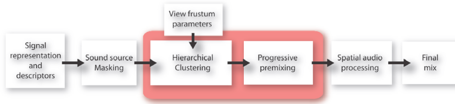
Figure 2.2: Overview of our overall sound rendering pipeline. In particular, we introduce a sound source clustering metric that better handles visible sources.
