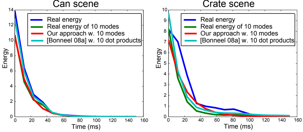
Figure 5.2: Plot of the instant energies computed with our approach (red), our previous energy computation (Chapter 3) (cyan), and the reference (blue), over the length of an impact sound on two scenes. Also shown the reference energy computed with 10 modes, simulating what our approach computes. Note that our approximation is much more efficient. Left: “Cans” sequence, right “Crates” sequence.
