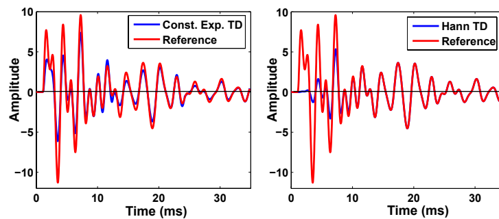
Figure 3.3: Comparison of Constant Exponential Approximation in the time domain (TD) and Hann window reconstruction in the TD, with the reference for the sharp sound of a falling box.
