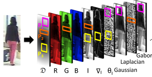
Fig. 3.4: A meta covariance feature space. Example of three different covariance features. Every covariance is extracted from a region ( P ), distance layer ( \mathcal{D} ) and three channel functions (e.g. bottom covariance feature is extracted from region P_3 using layers: \mathcal{D} , I -intensity, \nabla_I -gradient magnitude and \theta_I -gradient orientation).
