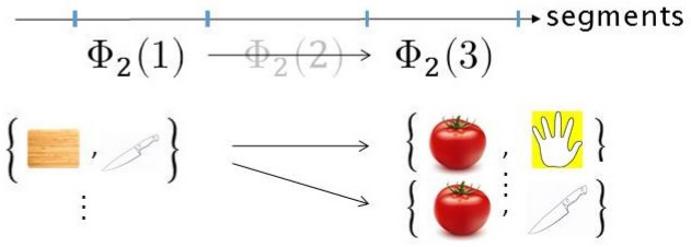
Figure 1. Semi-supervised learning of a video representation: 1) video temporal segmentation, 2) concept recognition 3) composite concept generation per time segment, 4) Temporal composite generation between segments.
