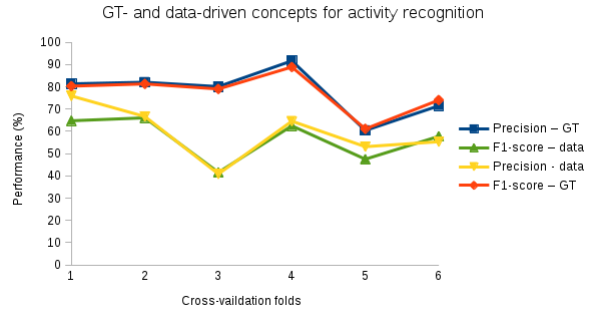
Figure 3. Complex activity recognition with annotated (blue and red lines) and automatically detected concepts (yellow and green lines) according to precision and f_1 -score indexes.
