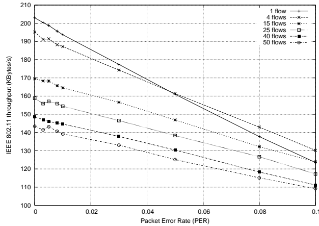
Figure 18: Throughput of 802.11 in noisy channel
