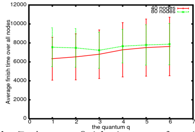
Fig. 7. Average finish time as a function of the chosen quantum
