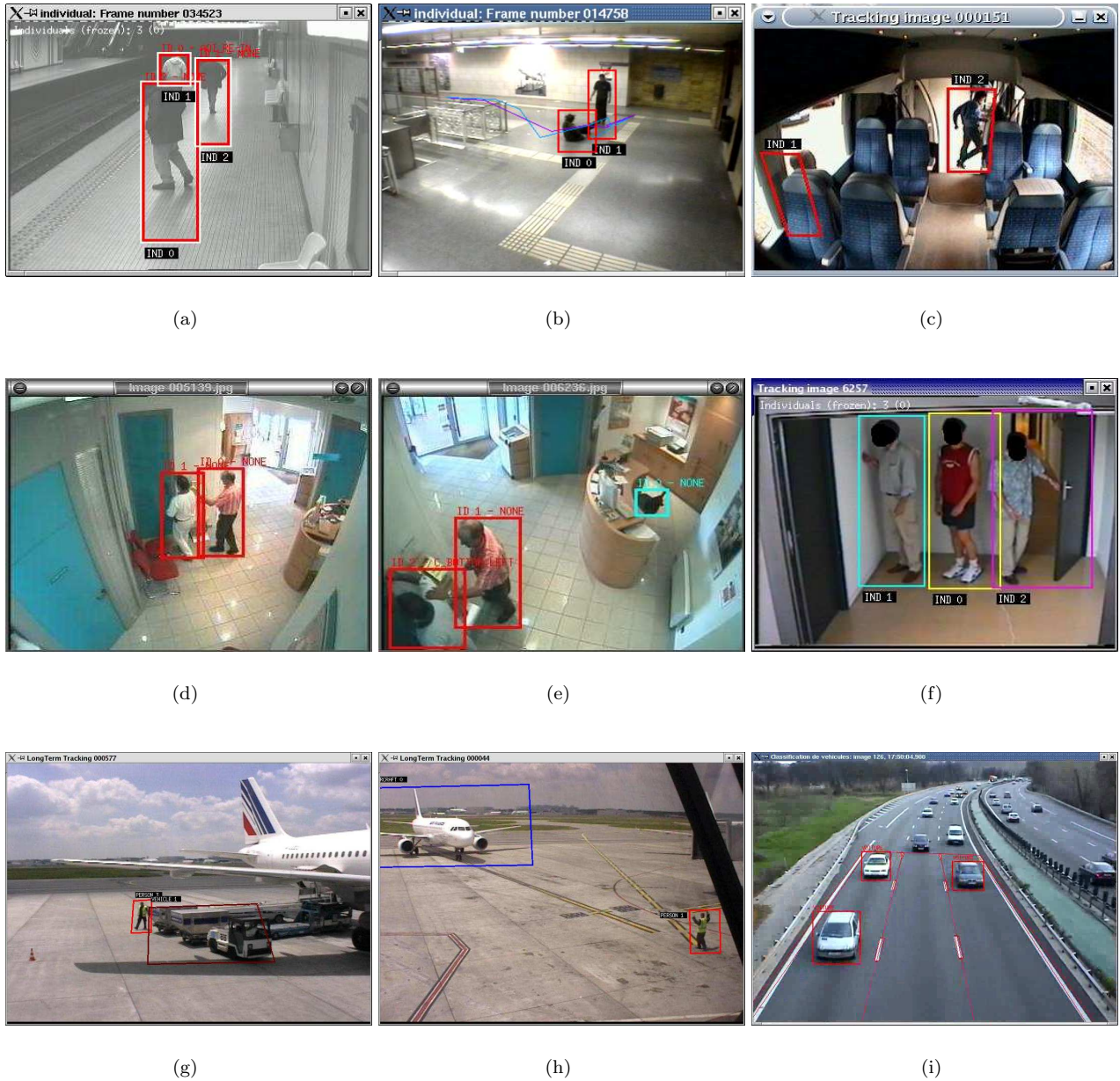
Fig. 1. This figure shows six Activity Monitoring Systems (AMS) derived from VSIP to handle different applications. Image 1(a) illustrates a metro monitoring application system running on black and white cameras of the YZER station in Brussels. Image 1(b) illustrates the same system but analyzing images from a color surveillance camera of the SAGRADA FAMILIA station in Barcelona. Image 1(c) illustrates a system for unruly behaviors detection inside trains. Images 1(d) and 1(e), taken with 2 synchronized cameras with overlapping field of view working in a cooperative way, illustrate a bank agency monitoring system detecting an abnormal “bank attack” scenario. Image 1(f) illustrates a single-camera system for a lock chamber access control application for building entrances. Images 1(g) and 1(h) illustrate an application for aprons monitoring on airports; this application combines a total of 8 surveillance cameras with overlapped fields of view. Finally, image 1(i) illustrates an highway traffic monitoring application.
