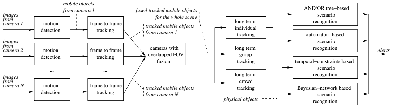
Fig. 2. This figure shows the global structure of the activity monitoring platform. First, a motion detection step followed by a frame to frame tracking is made for each camera. Then the tracked mobile objects (objects from camera i ) coming from different cameras with overlapping fields of view are fused into a unique representation for the whole scene. Depending on the chosen application, a combination of one or more of the available trackers (individuals, groups and crowd tracker) is used. The results are passed to the behavior recognition algorithms, which combine one or more of the following algorithms, depending on the scenarios to recognize: automaton based, Bayesian-network based, AND/OR tree based and temporal constraints based recognition algorithm. Finally the system generates the alerts corresponding to the predefined recognized scenarios.
