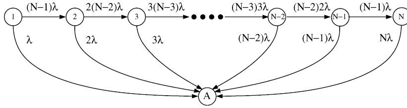
Fig. 2. Unrestricted multicopy protocol: transition diagram of the Markov chain for the number of copies.
