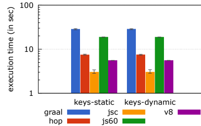
Figure 9. Comparing the raw performance of JavaScript implementations for static and dynamic property names. Smaller is better; log scale.
