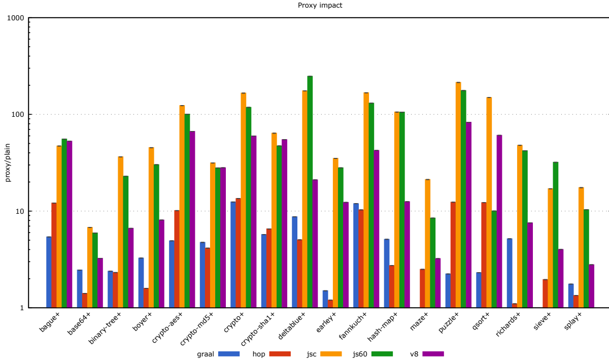
Figure 5. Impact of using proxies on performance. Each bar represents the ratio between the original test and the proxied version. Smaller is better; log scale.
