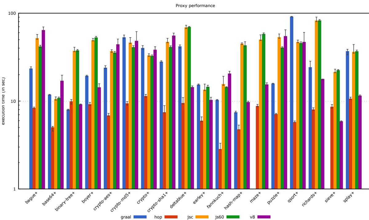
Figure 4. Comparison of proxy performance. Bars represent the mean of 30 execution times for each tested system and for each test. The bars for each implementation are in the same order as in the legend. Smaller is better; log scale.
