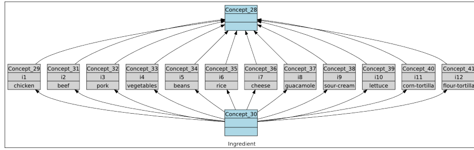
Fig. 2. The concept lattice for ingredients of the RCF in Table 1.
