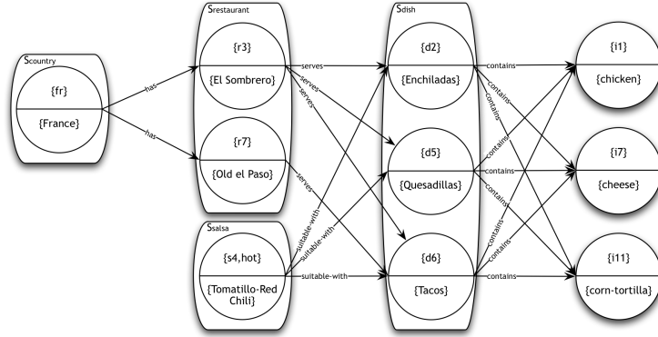
Fig. 5. The subgraph containing interesting objects for the relational query example.
