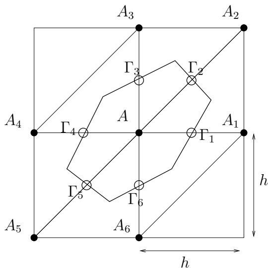
Figure 2: A particular mesh.
