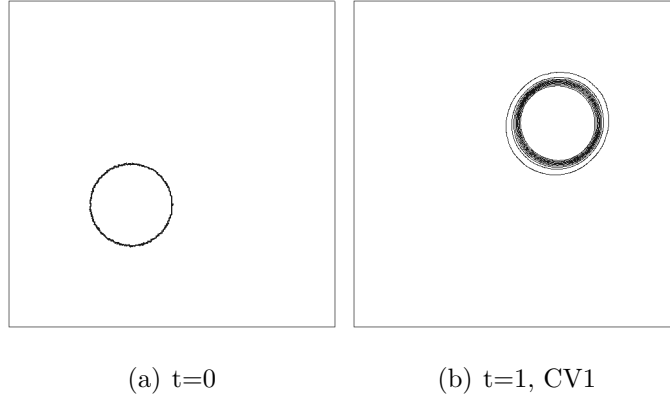
Figure 6: Density contours of a discontinuous function at t = 0 (left) and t = 1 (right).
