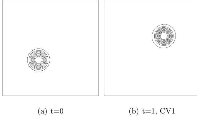
Figure 5: Density contours of a regular function at t = 0 (left) and t = 1 (right).
