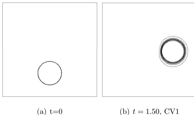
Figure 8: Density contours of a discontinuous function at t = 0 (left) and t = 1.50 (right).
