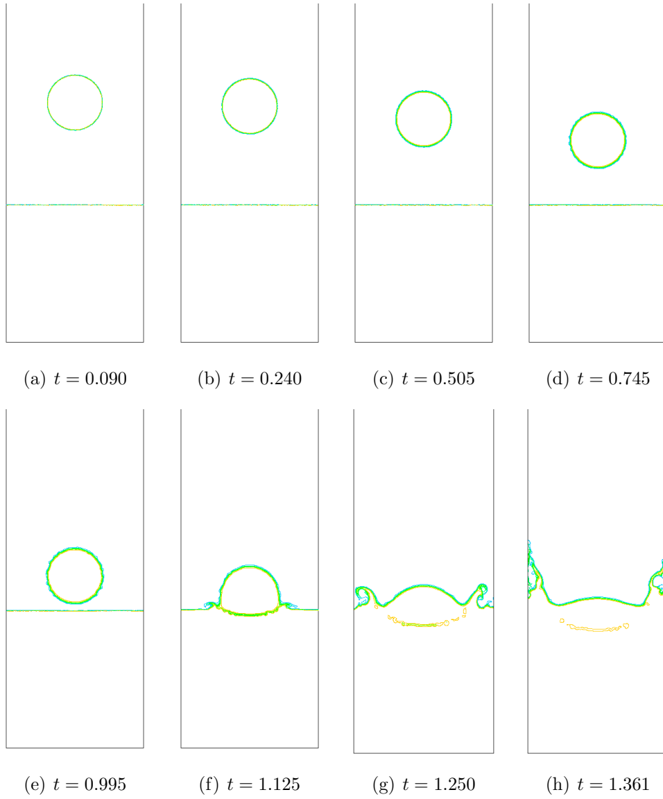
Figure 10: \rho_M = 1000 , h_{min} = 1/400 , density contours = [200, 350, 400, 450, 500, 550, 600, 650, 800].
