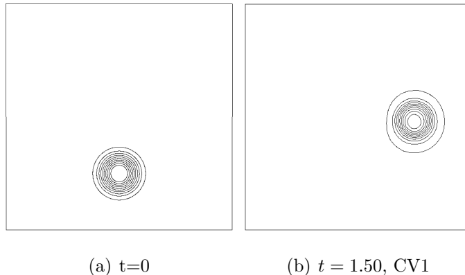
Figure 7: Density contours of a regular function at t = 0 (left) and t = 1.50 (right).
