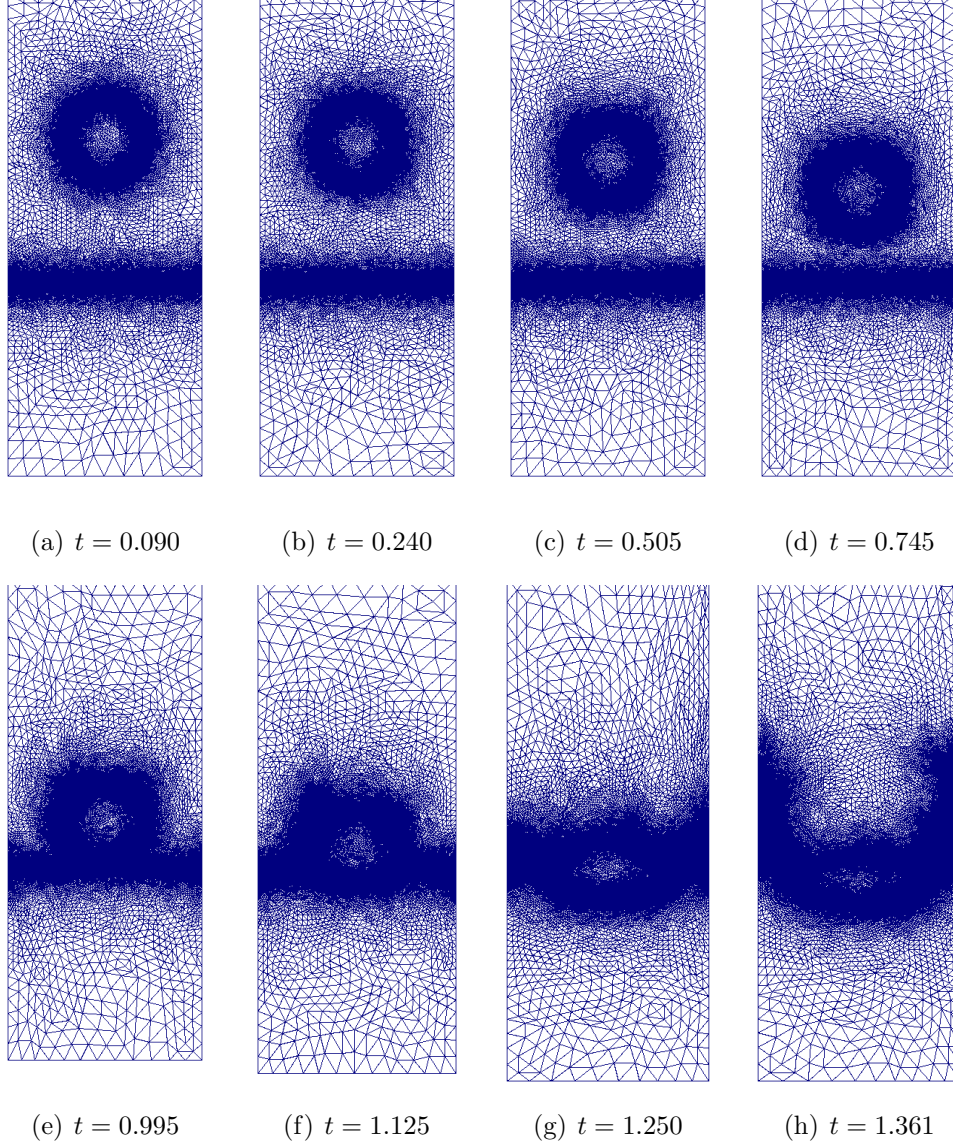
Figure 11: \rho_M = 1000 , h_{min} = 1/400 , meshes.
