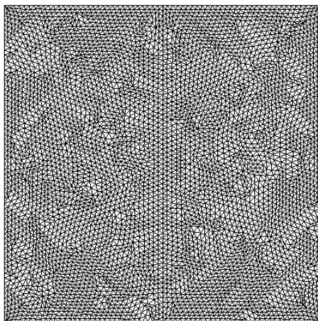
Figure 4: Example of unstructured mesh used without any adaptive process : Level 1.
