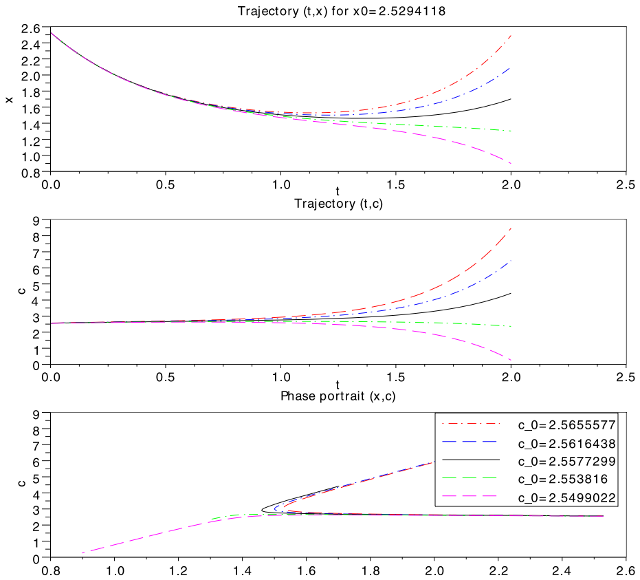
Fig. 4 Trajectories issued from x_0 = 2.53 and several values of c_0 around the estimated value \tilde{c}_0 = 2.57
