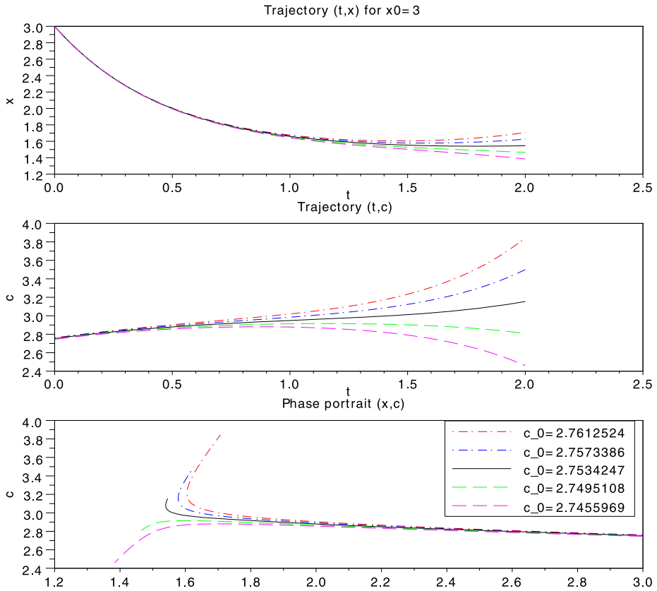
Fig. 2 Trajectories issued from x_0 = 3 and several values of c_0 around the estimated value \tilde{c}_0 = 2.75
