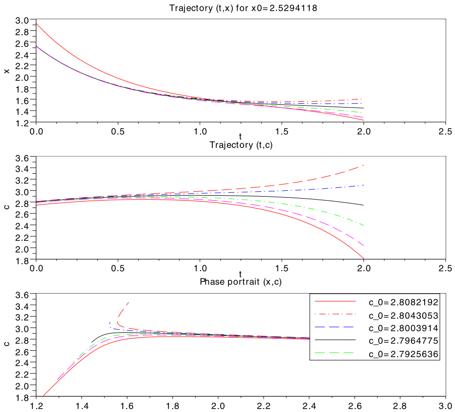
Fig. 3 Trajectories issued from x_0 = 2.53 and several values of c_0 around the estimated value \tilde{c}_0 = 2.81
