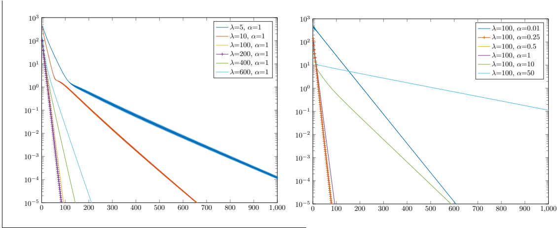
Fig. 11 Test 1, Mesh 1 1 , second Schwarz algorithm. Left : optimization of \lambda , with \alpha = 1 , \beta = 10^{-2} . Right : optimization of \alpha , with \lambda = 100 , \beta = 10^{-2} .
