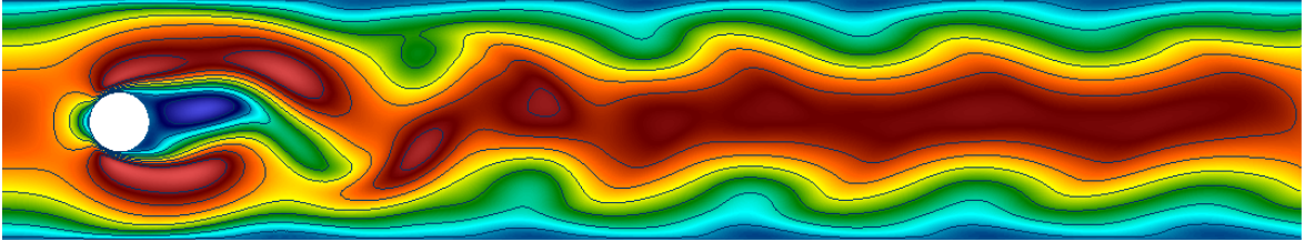
Fig. 24 First component of the velocity solution to the Navier-Stokes problem on \Omega , obtained at the 388 th iteration of the Schwarz algorithm, at T = 6\text{s} , in the case of 2 subdomains.
