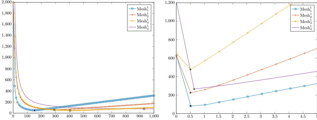
Fig. 12 Test 1, (\text{Mesh}_m^1)_m , m = 1, 2, 3, 4 . Left : optimization of \lambda to obtain an error of order 10^{-5} , with \alpha = 1, \beta = 10^{-1} . Right : optimization of \alpha to obtain an error of order 10^{-5} , with \lambda = 100, \beta = 10^{-1} .
