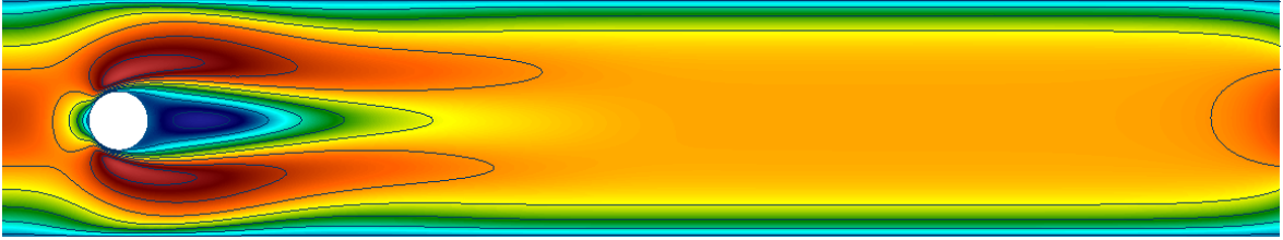
Fig. 19 First component of the velocity solution to the Navier-Stokes problem on \Omega at T = 2\text{s} .
