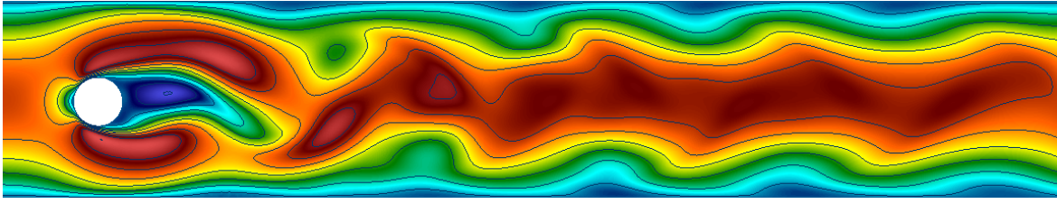
Fig. 26 First component of the velocity solution to the Navier-Stokes problem on \Omega , obtained at the 663 th iteration of the Schwarz algorithm, at T = 6s , in the case of 5 subdomains.
