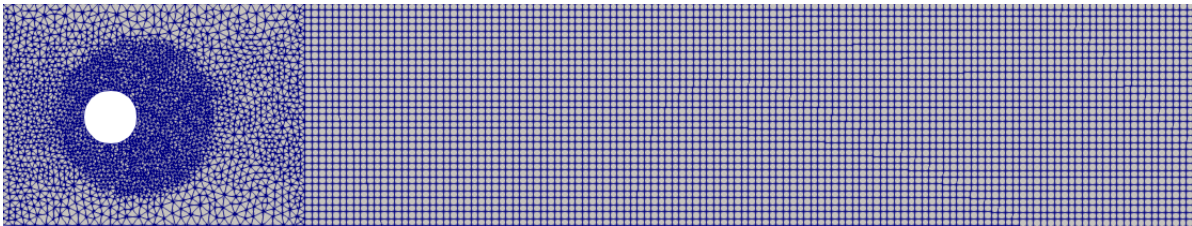
Fig. 18 Mesh on the domain \Omega of Fig. 17. The number of primal cells is 34634; 18250 in the left domain, 16384 in the right one.
