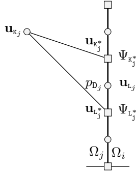
Fig. 5 The unknowns on a diamond on the interface for the subdomain \Omega_j .
