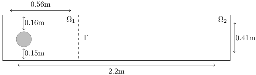
Fig. 17 Domain \Omega = [0, 2.2] \times [0, 0.41] , decomposed in \Omega_1 = [0, 0.56] \times [0, 0.41] and \Omega_2 = [0.56, 2.2] \times [0, 0.41] .
