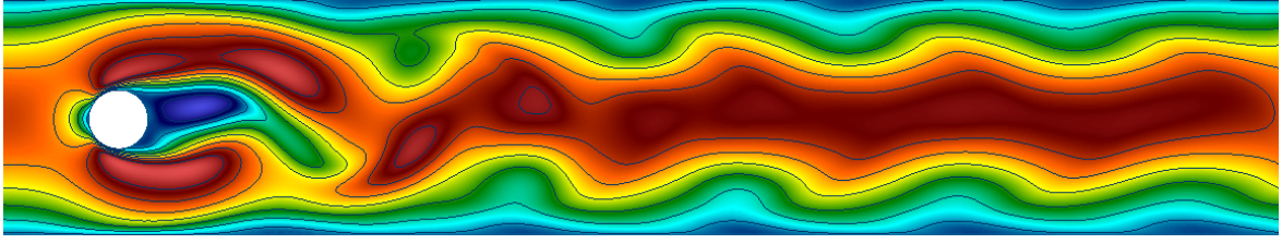
Fig. 21 First component of the velocity solution to the Navier-Stokes problem on \Omega at T = 6s .
