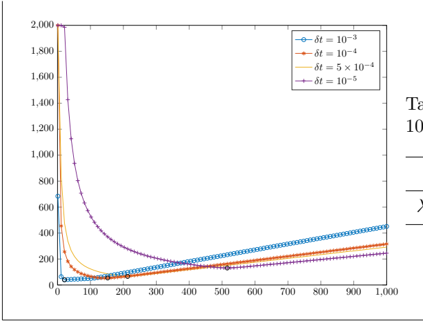
Fig. 14 Left : Test1, optimization of \lambda for different time steps to obtain an error of order 10^{-5} , \alpha = 1 and \beta = 10^{-1} . Right : Summary table of the optimal values of \lambda .
