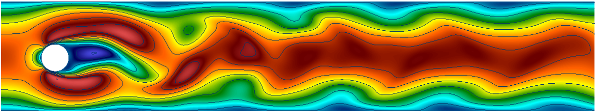
Fig. 25 First component of the velocity solution to the Navier-Stokes problem on \Omega , obtained at the 484 th iteration of the Schwarz algorithm, at T = 6\text{s} , in the case of 4 subdomains.
