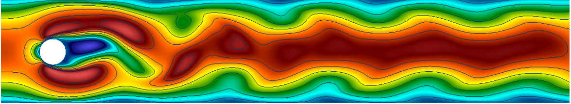
Fig. 22 First component of the velocity solution to the Navier-Stokes problem on \Omega , obtained at the 689 th iteration of the Schwarz algorithm, at T = 6s .
