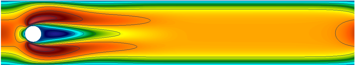
Fig. 20 First component of the velocity solution to the Navier-Stokes problem on \Omega , obtained at the 559 th iteration of the Schwarz algorithm, at T = 2\text{s} .
