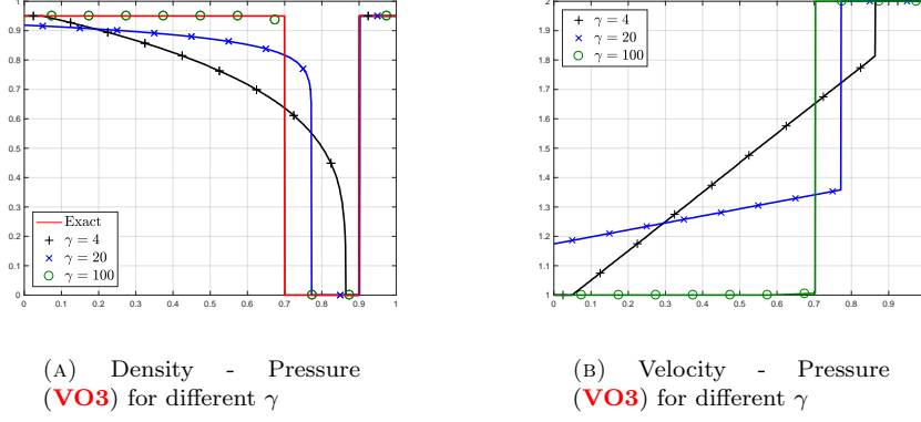
FIGURE 3. Numerical results in the case of decongestion (17)–(18). Pressure (VO3) for different values of \gamma . Density (left) and velocity (right) at final time T = 0.2 : \gamma = 4 (black), \gamma = 20 (blue) and \gamma = 100 (green). The simulations are performed with the implicit-explicit scheme and the exact solution is plotted in red.
