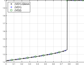
(B) Velocity - Pressures (VO1) and (VO2)
