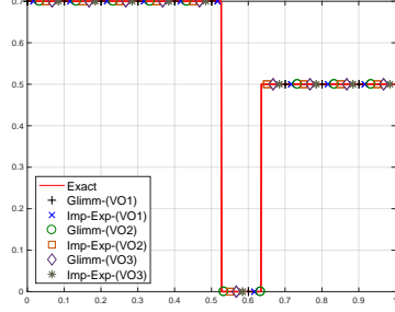
(A) Density at t=0.27
