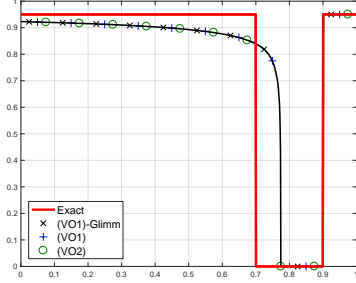
(A) Density - Pressures (VO1) and (VO2)
