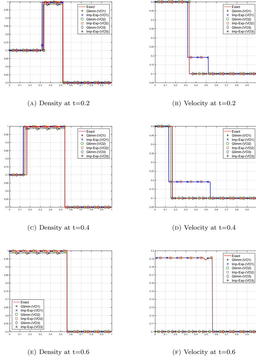
FIGURE 12. Comparison of the numerical scheme and velocity offset for the initial data (AI). We display the densities on the left and the velocities on the right, at t = 0.2 (top), t = 0.4 (middle) and t = 0.6 (bottom). Glimm scheme with pressures (VO1) (in black), (VO2) (in green) and (VO3) (in purple); implicit-explicit scheme with pressures (VO1) (in blue), (VO2) (in orange) and (VO3) (in grey). The exact solution is plotted in red.
