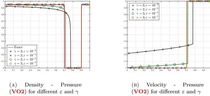
FIGURE 4. Numerical results in the case of decongestion (17)–(18). Pressure (VO2) for different values of \varepsilon and \gamma . Density (left) and velocity (right) at final time T = 0.2 : (VO2) for \gamma = 2, \varepsilon = 10^{-3} (black), \gamma = 2, \varepsilon = 10^{-5} (blue), \gamma = 3, \varepsilon = 10^{-5} (green) and \gamma = 3, \varepsilon = 10^{-7} (orange). The simulations are performed with the implicit-explicit scheme and the exact solution is plotted in red.
