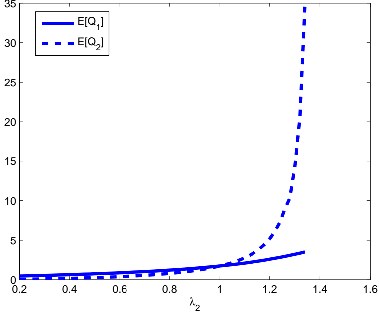
Fig. 5 The expected queue lengths of the orbit queues as functions of \lambda_2 ( \lambda_1 = 1 , \mu_1 = \mu_2 = 2 , \mu = 4 ).
