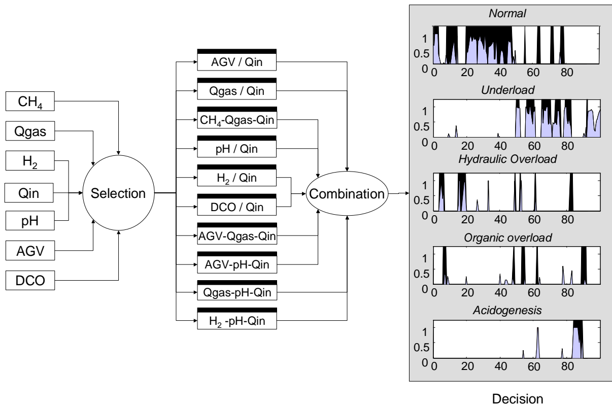
Figure 4: Illustration of the results provided by the TELEMAC fault detection and diagnosis system.
