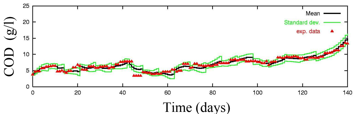
Figure 3. Software sensor validation: off-line soluble COD measurements ( \Delta ) are compared to the predictions of the software sensors (average predicted value and confidence interval).
