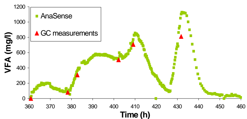
Figure 2. Validation of the AnaSense sensor dedicated to the measurement of VFA, bicarbonate, total and partial alkalinity.
