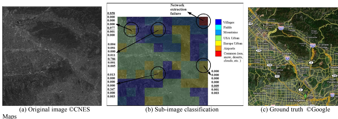
Figure 4 : Large image indexing
