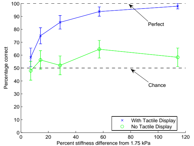
Fig. 7. User stiffness discrimination ability
