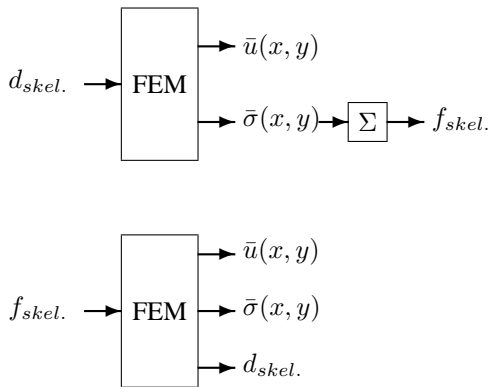
Fig. 2. Finite element models.
