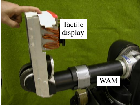
Fig. 4. Entire system
