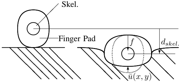
Fig. 1. Cross section through finger and compliant slab of material. Left: prior to application of contact force; Right: finger indenting material
