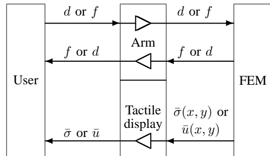
Fig. 3. Interaction between user and FEM
