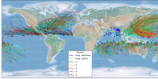
(a) Tracking database: more than 3000 tropical/extra-tropical storm tracks since 1979. Dots = initial position, colors = maximal strength (Saffir-Simpson scale).
