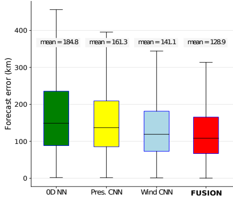
Figure 3: 24h-forecast results on the test set (storms coming from all oceanic basins), in distance between predicted and real location.
