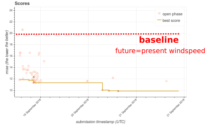
Fig. 6: Scores (RMSE) of the submissions wrt. time on the public leaderboard (cross-validation score using the online training set, score visible during the event).
