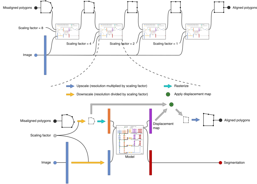
Fig. 4: Multi-resolution pipeline.
