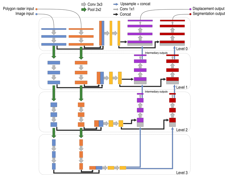
Fig. 2: Model architecture for one resolution. There are 4 different levels inside the network: one after each pooling operation in addition to the first level.
