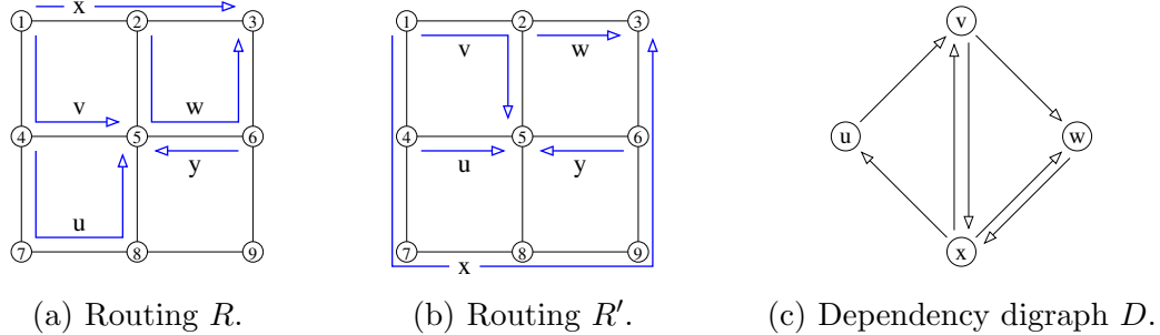
Fig. 2. Figs. 2(a) and 2(b) give two routings, R and R' , for the set of lightpaths \{u, v, w, x, y\} on the 3 \times 3 grid. Each link of the grid is symmetric and has capacity 1 (i.e. a single wavelength) in both directions. Fig. 2(c) presents the dependency digraph for switching from routing R to routing R' .
