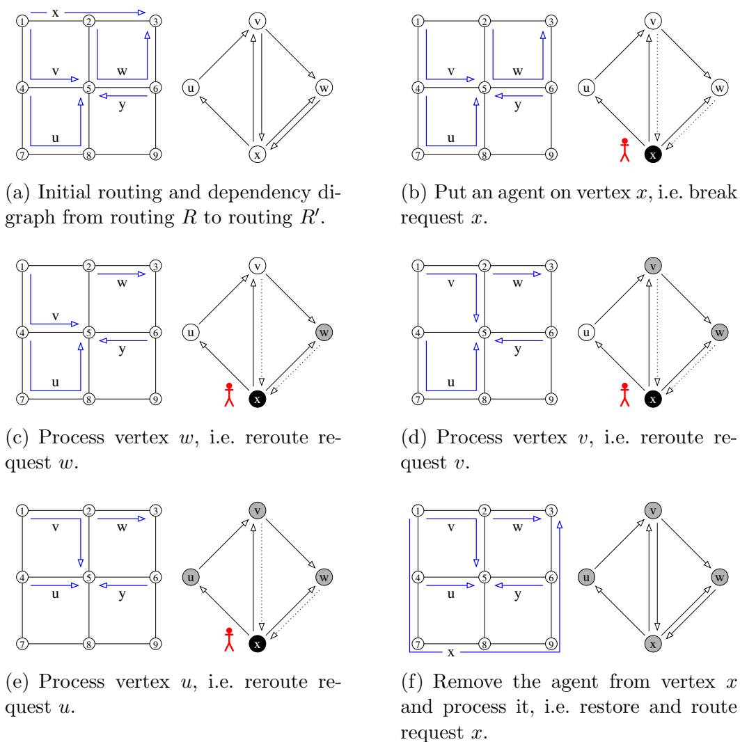
Fig. 3. Processing of the example of Fig. 2: processed vertices are in gray and vertices covered by an agent are in black. In Fig. 3(b), every vertex has at least one outneighbor in the initial state, so we must put an agent on some vertex. We choose vertex x in Fig. 3(b). Since vertex w now satisfies that all its outneighbors are either processed or covered by an agent, we process it in Fig. 3(c). Then we can process vertex v in Fig. 3(d) and vertex u in Fig. 3(e). Finally, we can process vertex x in Fig. 3(f), which frees the agent.
