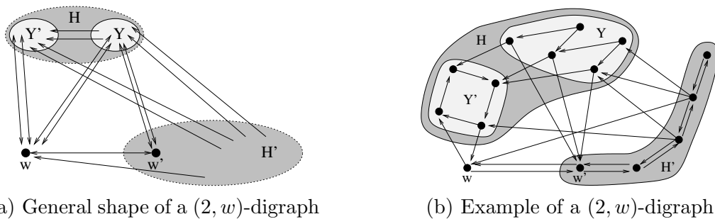
Fig. 7. The general shape and an example of a (2, w) -digraph.
