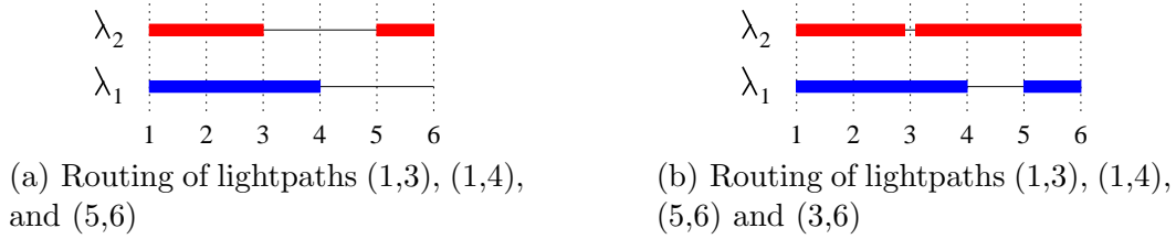
Fig. 1. Example of a blocked lightpath in a WDM network. The network topology is a 6-node-path with 2 wavelengths. In Fig. 1(a), the lightpath (3,6) will be rejected although the routing of Fig. 1(b) is possible, up to the rerouting of lightpath (5,6).
