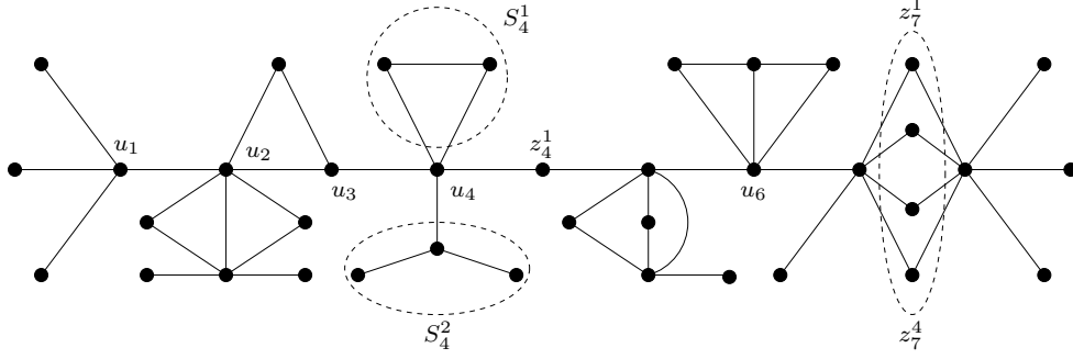
Fig. 6. A typical graph with process number 2.
