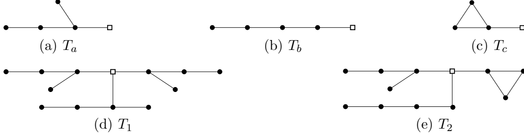
Fig. 5. T_1 and T_2 are two of the ten non-isomorphic minor-obstructions for 2-processed graphs obtained using three subgraphs chosen among T_a , T_b and T_c and merged at vertex \square .
