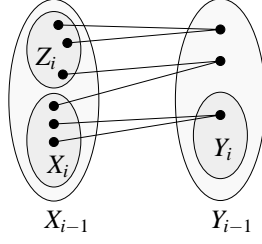
Figure 2: X_i = X_{i-1} \setminus Z_i and Y_i = Y_{i-1}^{X_i} .
