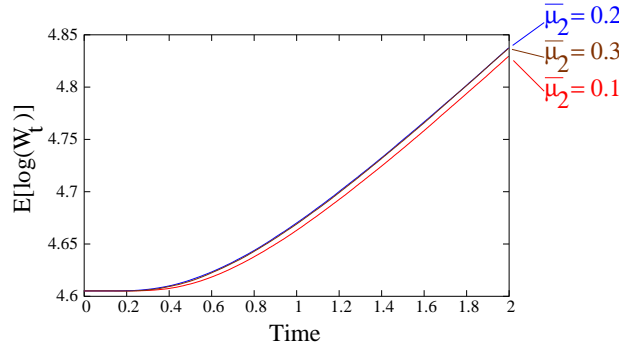
Fig. 4. Error on \mu_2 for the optimal trader
