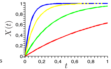
Fig. 2. The evolution of X(t) as a function of t under the best work conserving policy for \lambda = 1, 3, 8, 15 . The curves are ordered according to \lambda with the top curve corresponding to the largest \lambda etc.
