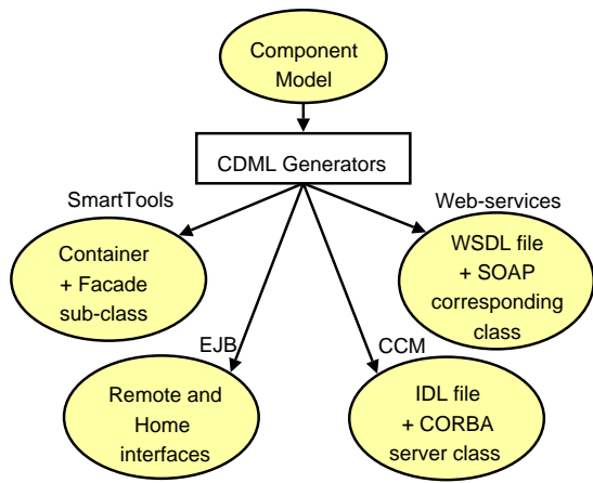
Figure 12: Component model transformations
