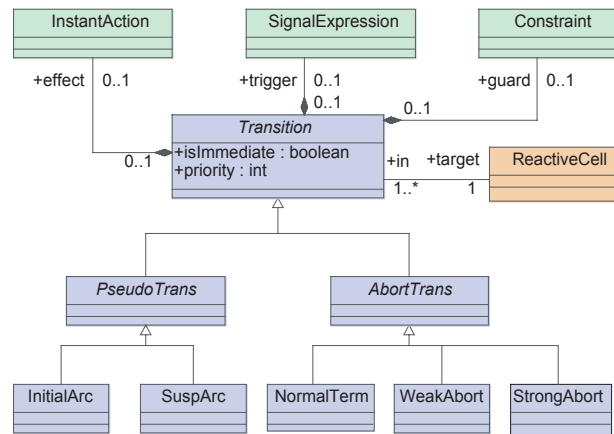
Fig. 6. SYNCCHARTS's Metamodel: Transitions.
