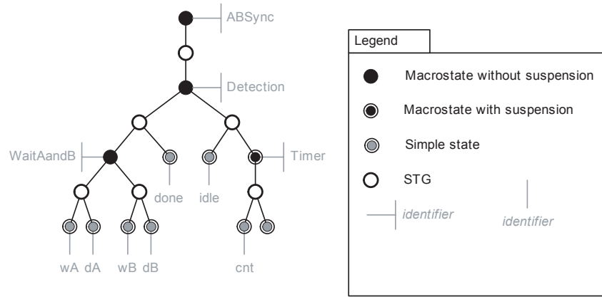
Fig. 7. Tree associated with a syncChart.
