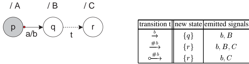
Fig. 3. Immediate Reactions: Behavior according to the type of preemption applied to state q, when p is active, and a occurs.
