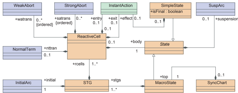
Fig. 5. SYNCCHARTS’s Metamodel: States.
