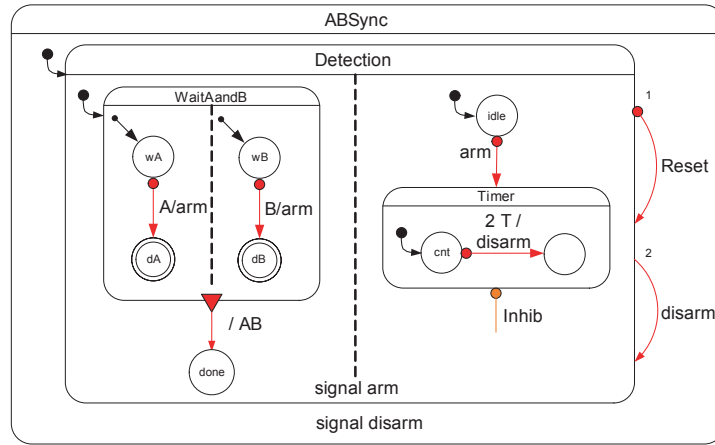
Fig. 1. A Typical SyncChart: This syncCharts specifies a detector of synchronized occurrences. Signal AB must be emitted when A and B have occurred, in any order, but “close enough” in time. “Close enough” means that there are at most two occurrences of T between the occurrences of A and B . Reset is a signal re-initializing signal. Finally, Inhib is a signal that enables “time suspension”: when Inhib is present, possible occurrences of T are ignored.
