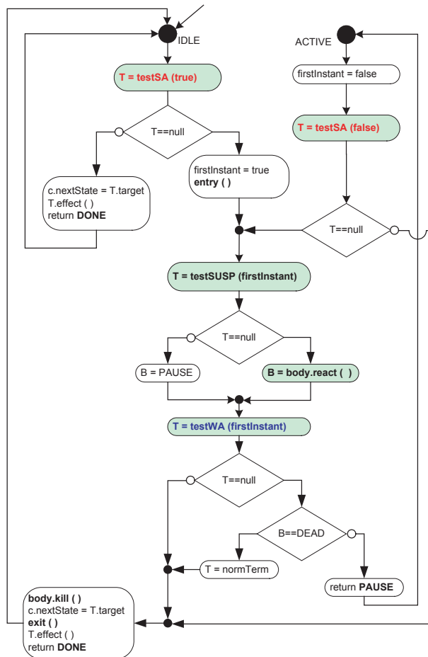
Fig. 8. ReactiveCell Reaction: ReactiveCell::react () method.
